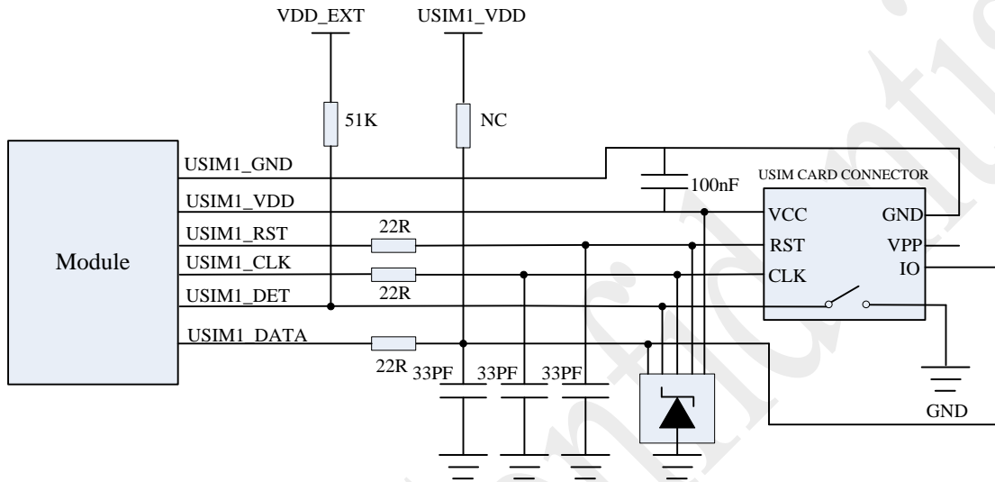
FIG. 12 Reference design drawing of the booth with hot-plug function
